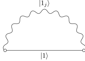
Fig. 10. The ground state energy of the harmonic oscillator is shifted by a transition to the first excited state accompanied by a virtual excitation of the j -th environmental mode
